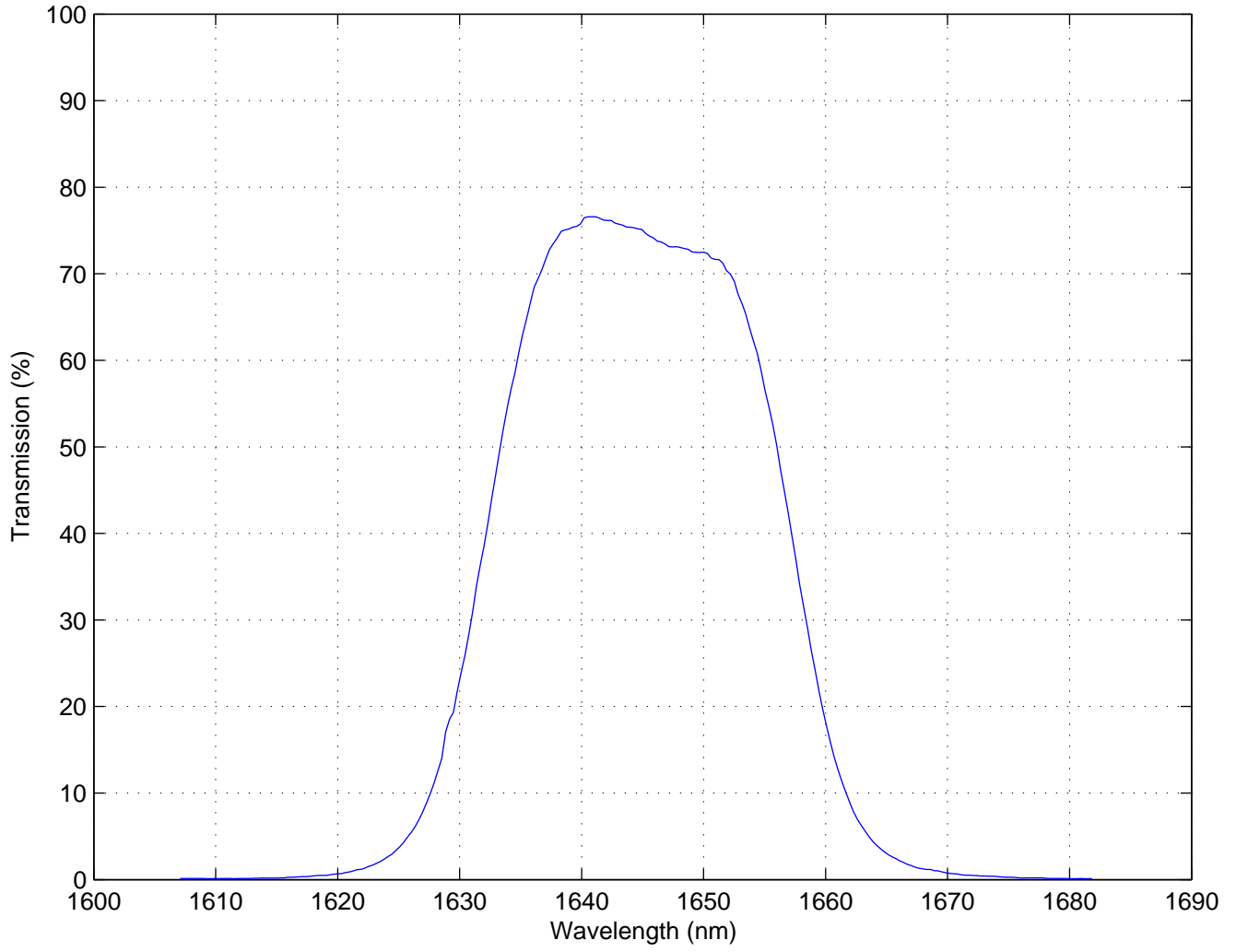
Filter #212, Fe II, vacuum wavelength, T=74K
