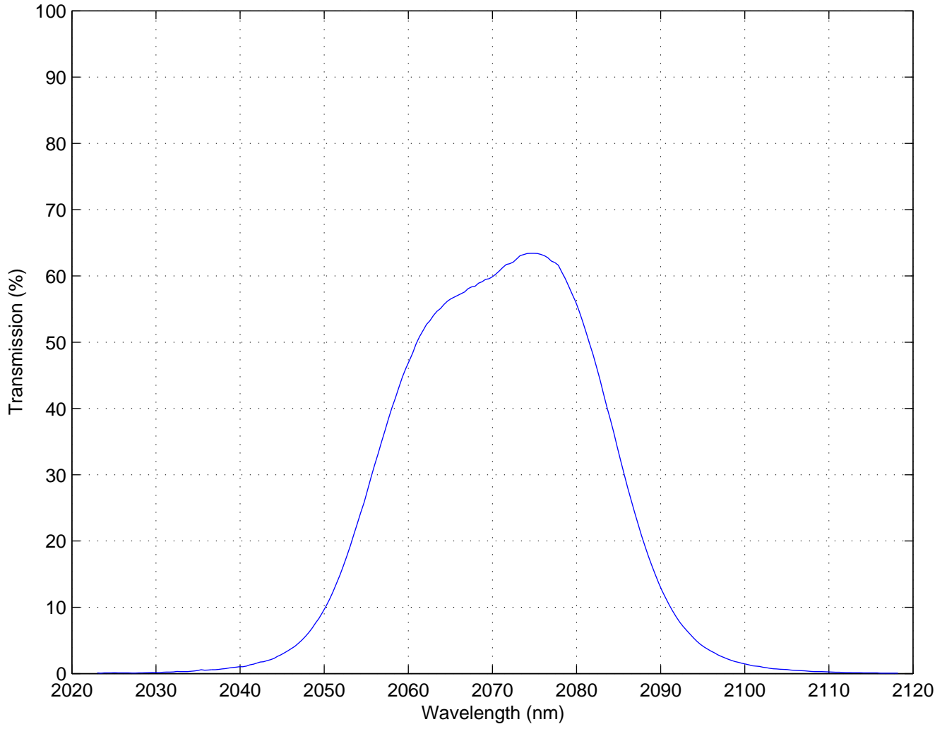
Filter #217, He I \lambda , vacuum wavelength, T=74K
