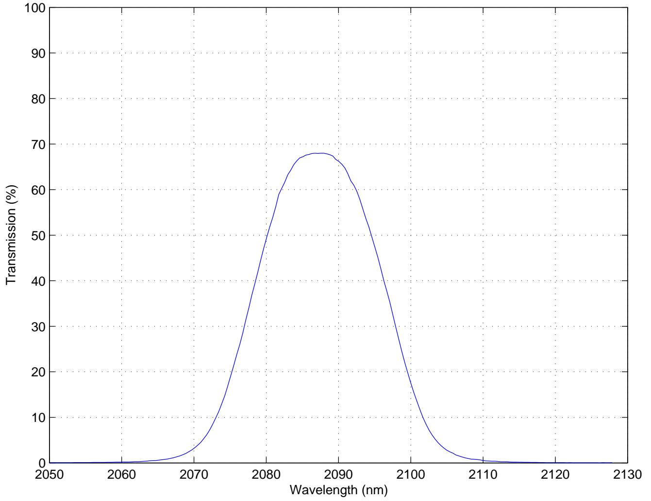
Filter #230, H2 continuum, vacuum wavelength, T=74K
